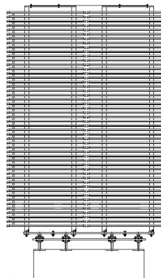
SECTION F-F
